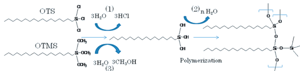
Scheme 1. Reaction Schemes of OTS and OTMS a
